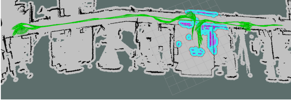
Figure 12.17: Best result obtained by AMCL on the Mini on record 007
