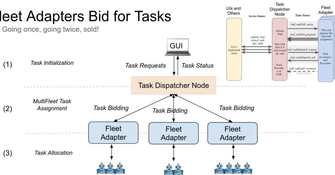
Figure 7.3: Open-RMF Bid Task
