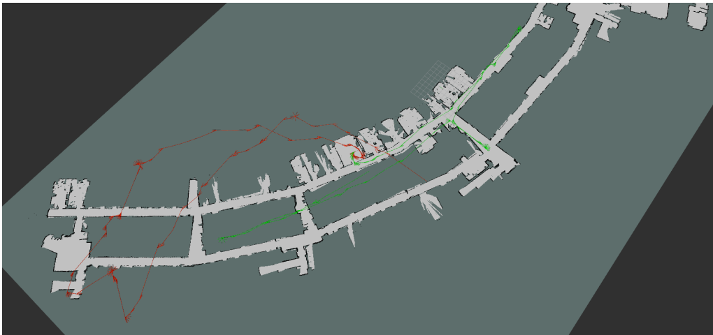
Figure 12.4: Mini odometry given by the robot (red) and odometry given by the robot_localization package
