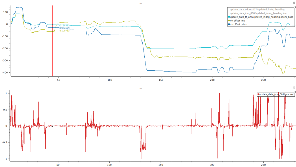
Figure 12.3: Heading result given by the sensors
