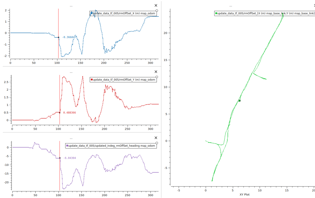
Figure 12.20: Plots of the best result for the Jobot with record 001
