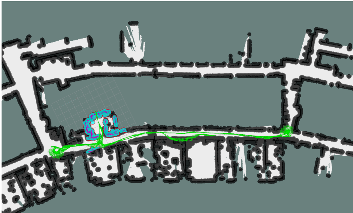
Figure 12.21: Result of the Jobot with record 002
