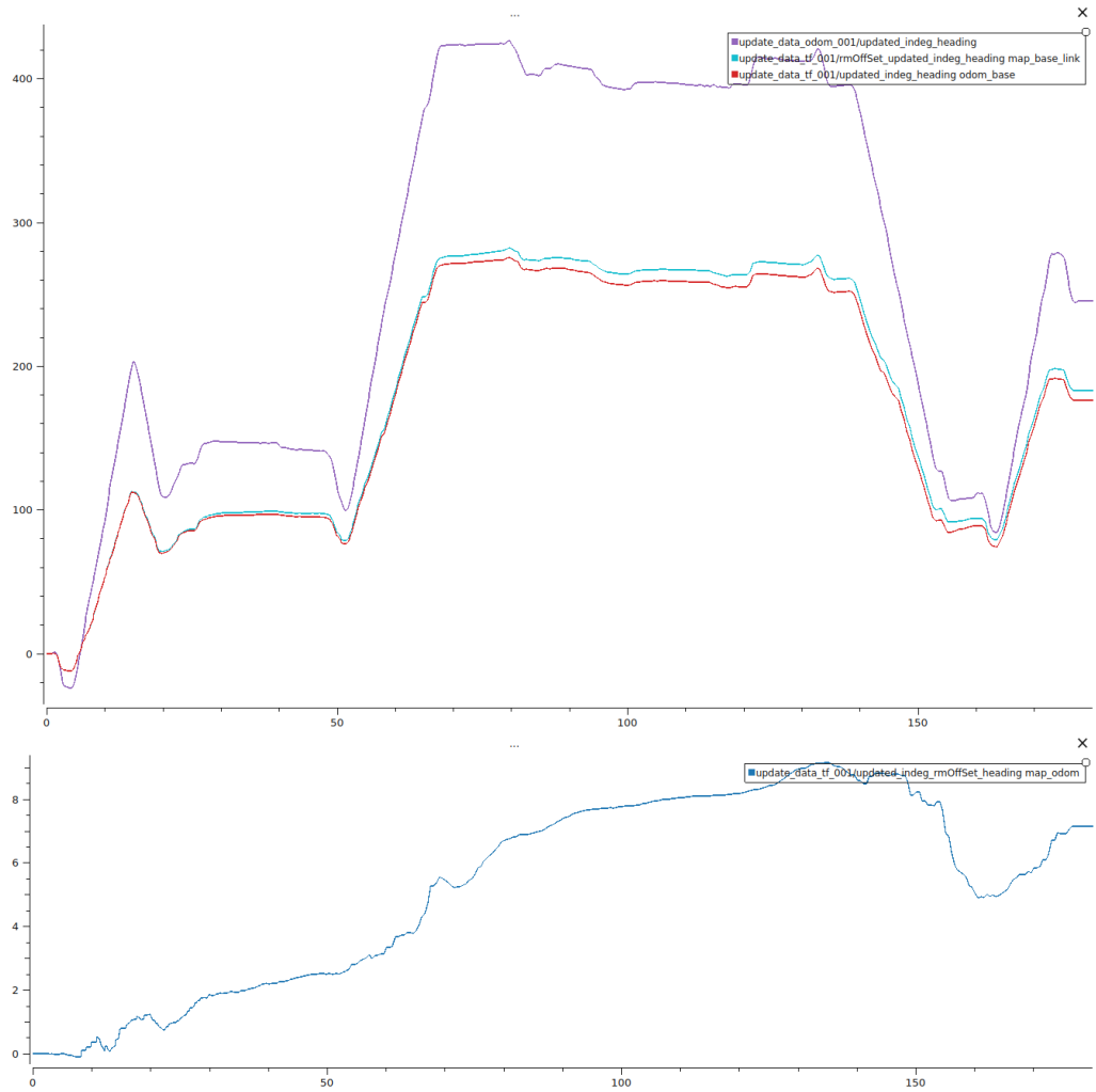
Figure 12.16: Heading correction for the Mini with AMCL
