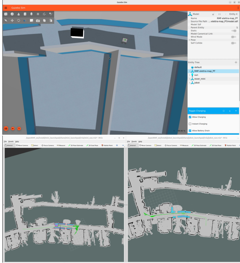
Figure 13.2: both robots simulated
