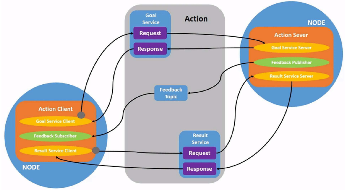
Figure 2.5: Action process
