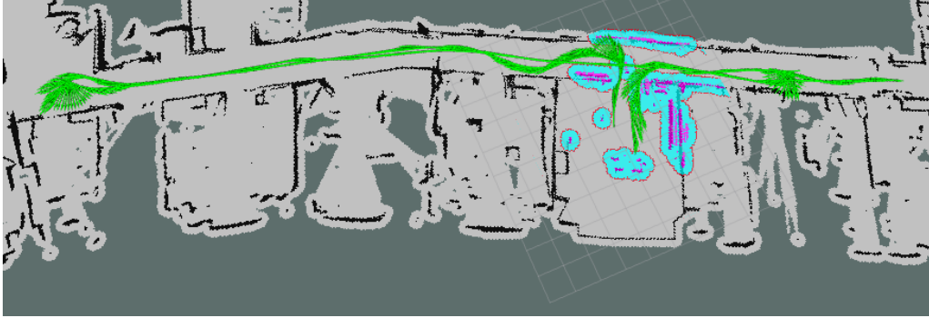
Figure 12.17: best result
