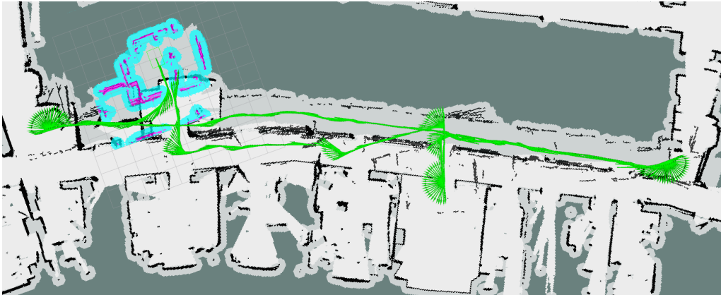
Figure 12.19: record1
