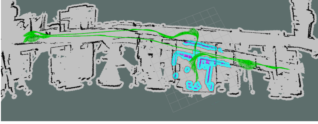
Figure 12.14: mini_ekf_no_correction_record007
