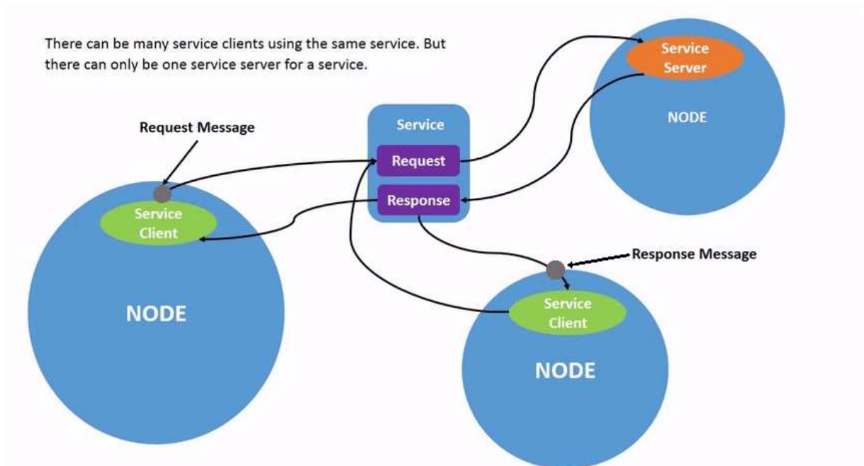
Figure 2.4: Service process
