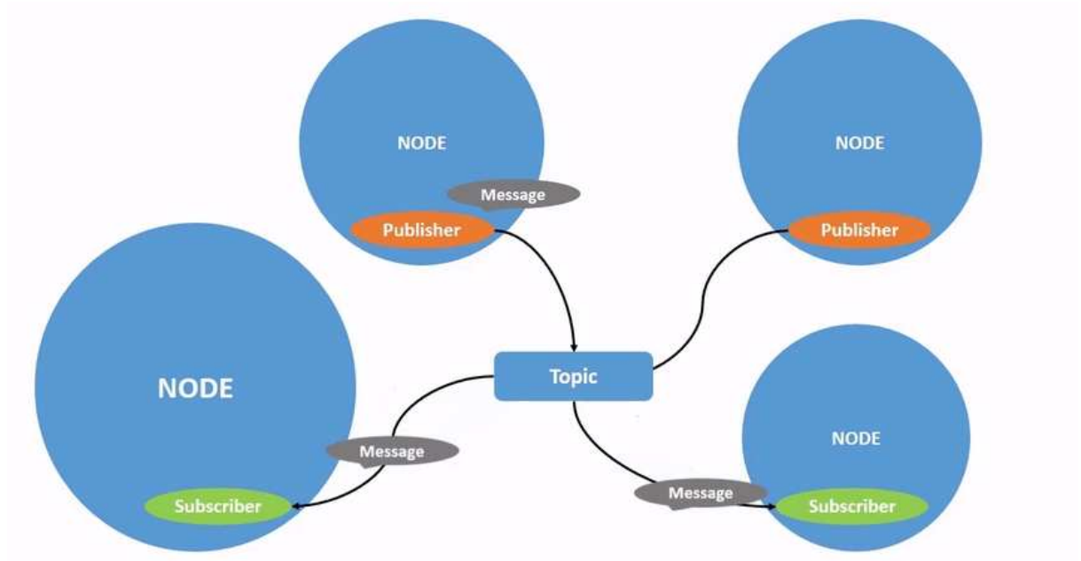
Figure 2.3: Topic process
