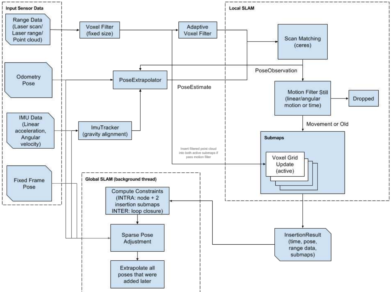
Figure 2.12: Cartographer Algorithm
