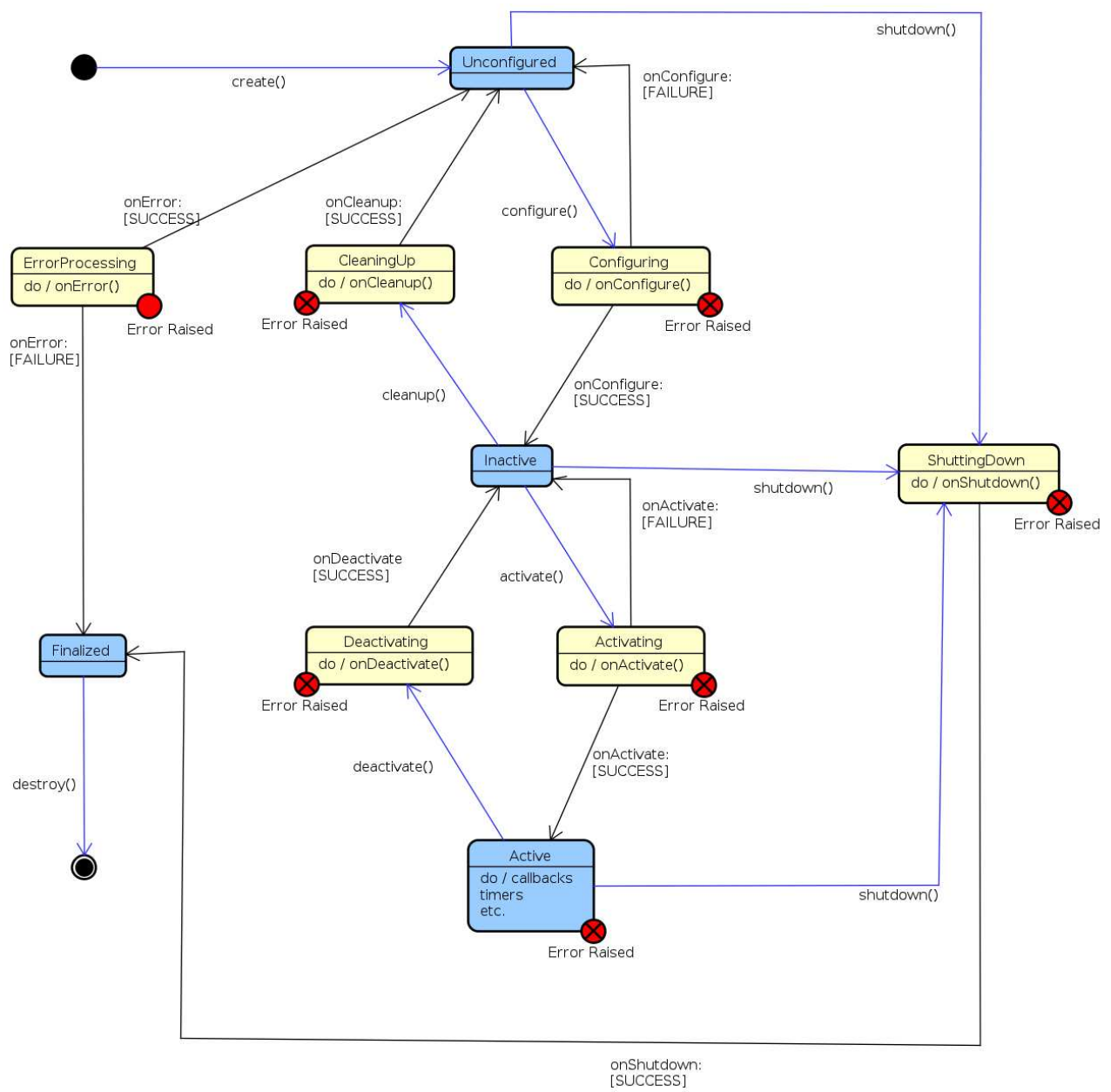
Figure 2.2: State Machine of LifecycleNode
