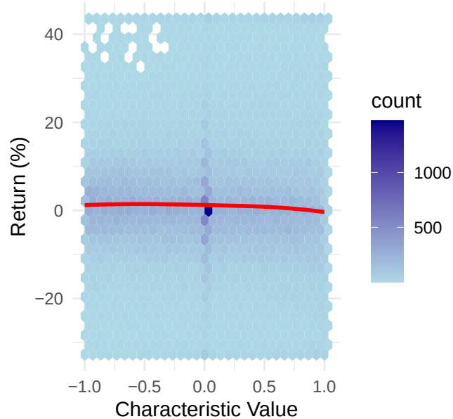
rank_ill
