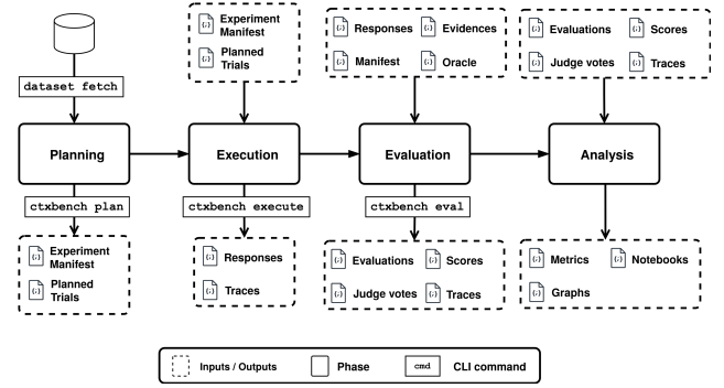
Figure 2: LLMContextBench workflow.
