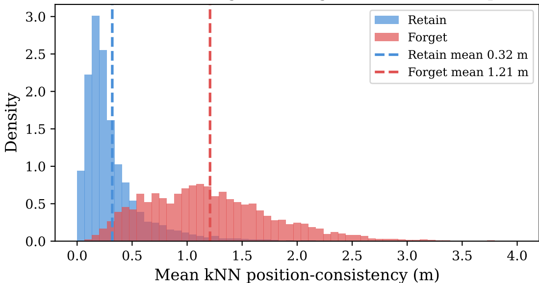
Contamination diagnosis: forget labels are corrupted
