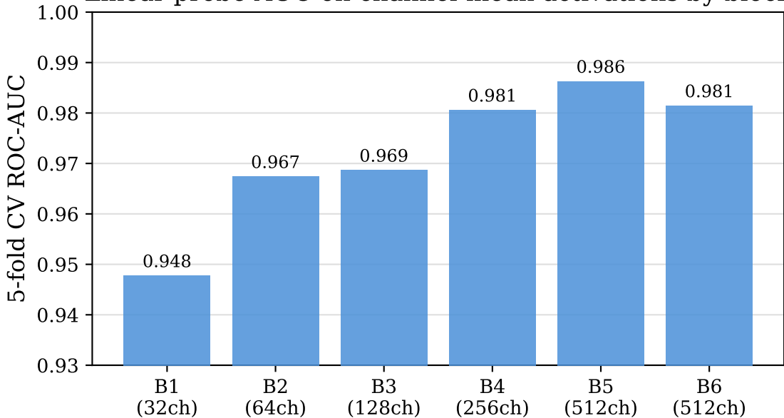
Linear probe AUC on channel-mean activations by block
