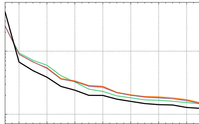
Stressed, (0.2, 1, 0.9)
