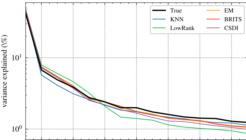
Sparse, rate 0.3
