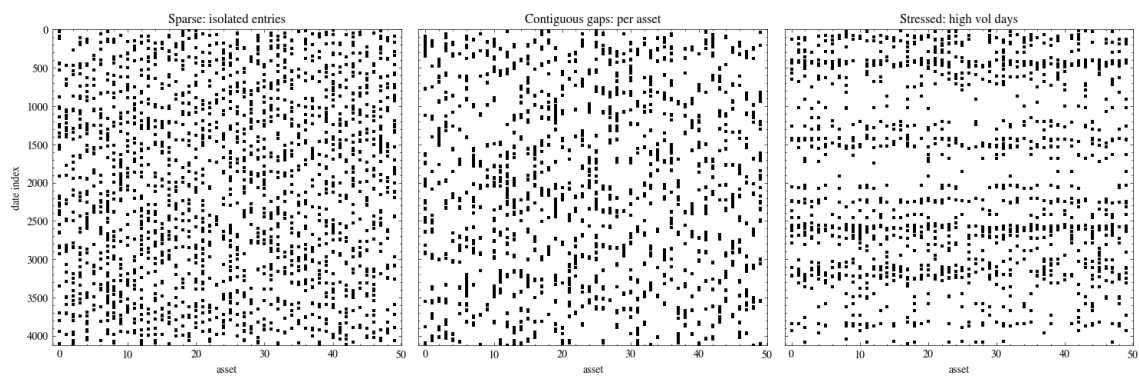
Figure 3.1: Examples of Imputed Data
