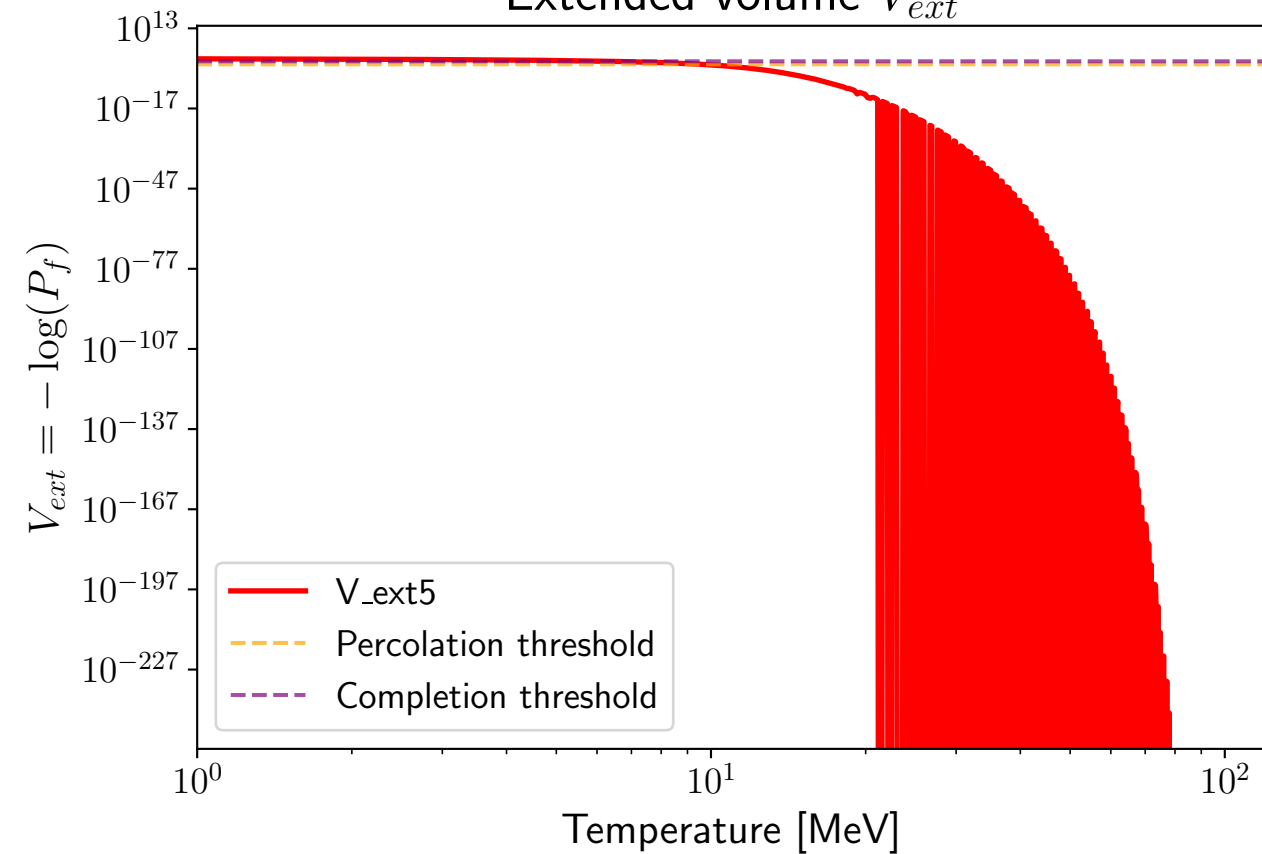
Extended volume V_{ext}
