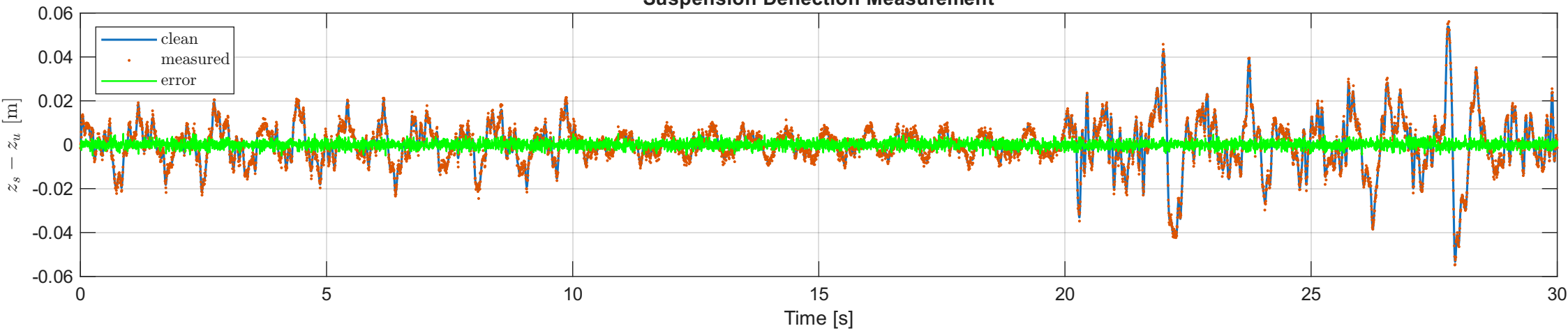
Suspension Deflection Measurement
