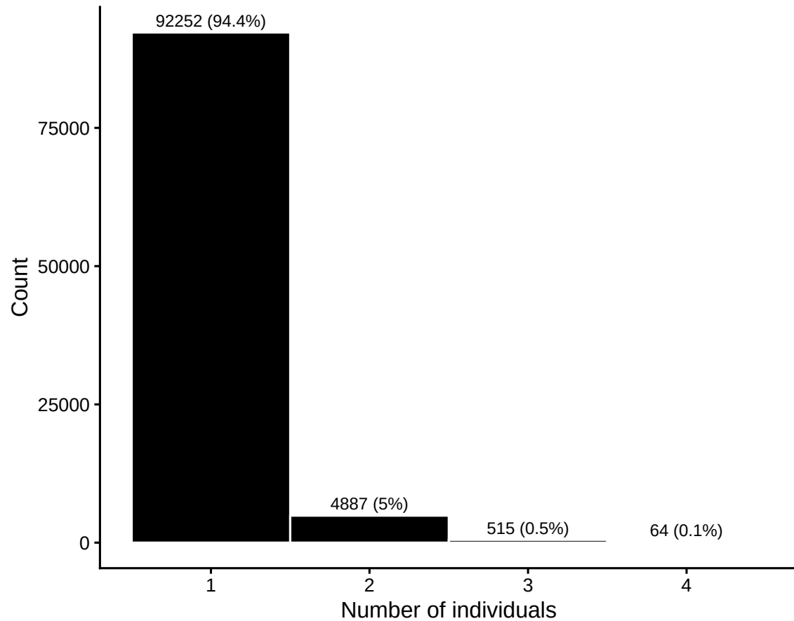
cluster_0.30 ... individuals per cluster
