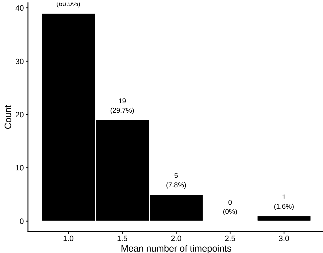
cluster_0.30 ... timepoints per prevalent cluster
