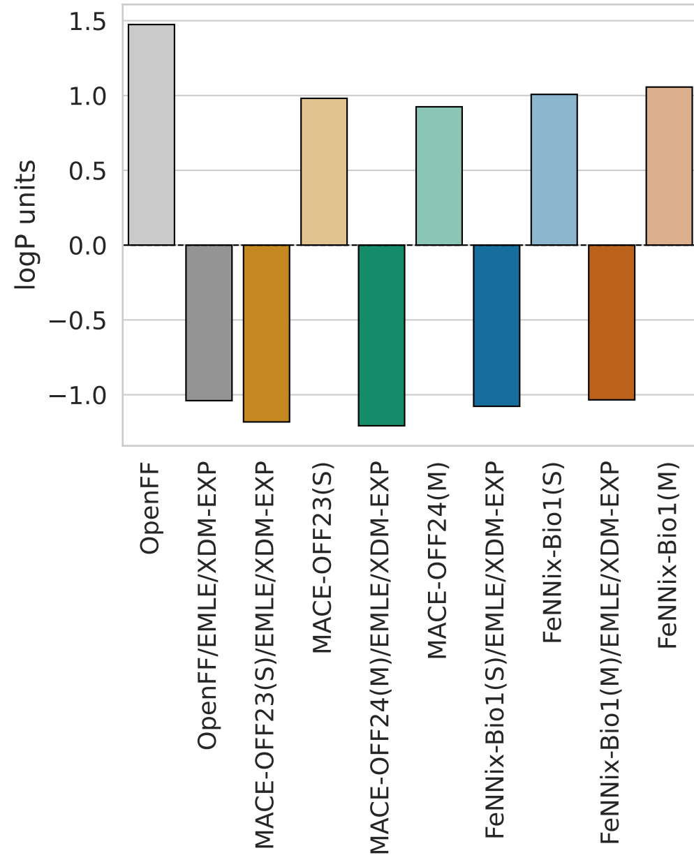
Bias
