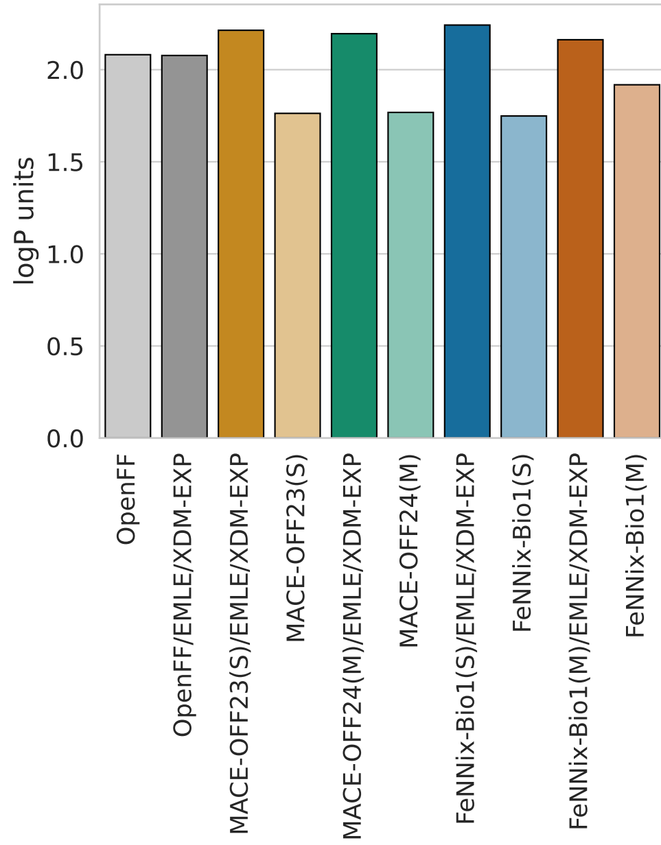
RMSE
