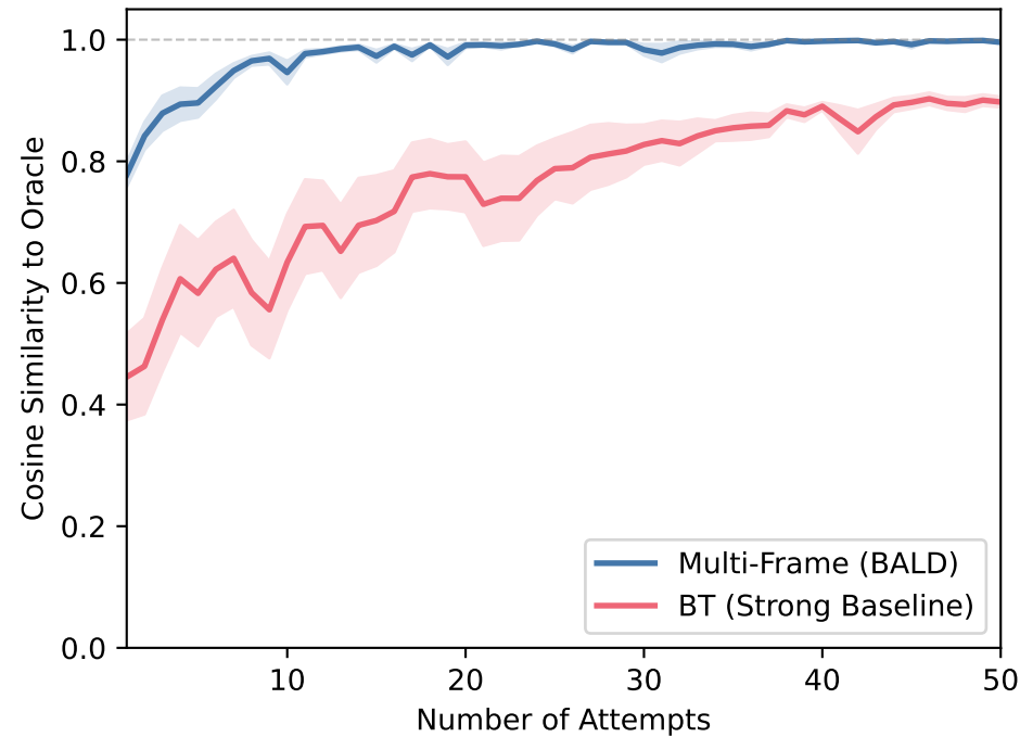
Convergence ( \tau=\tau'=0.25 , 15 trials)
