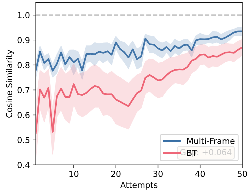
Query Selection: BALD
