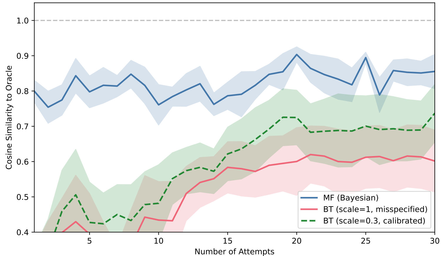
Effect of Likelihood Scale at \tau=\tau'=0 (Random Queries, 5 trials)
