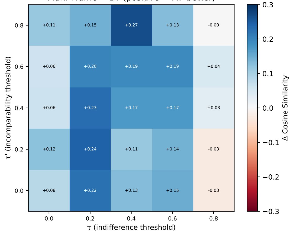
Multi-Frame – BT (positive = MF better)
