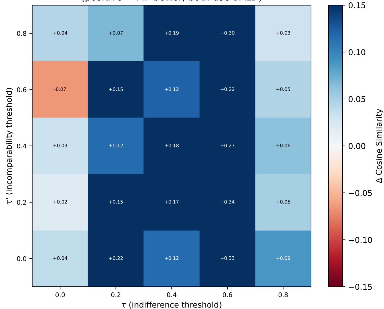
Multi-Frame – BT Laplace-BALD (positive = MF better, both use BALD)
