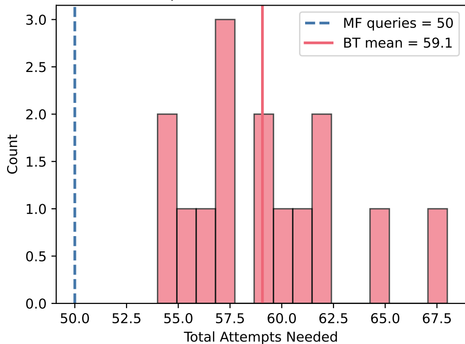
BT Attempts to Reach 50 Decisive Labels
