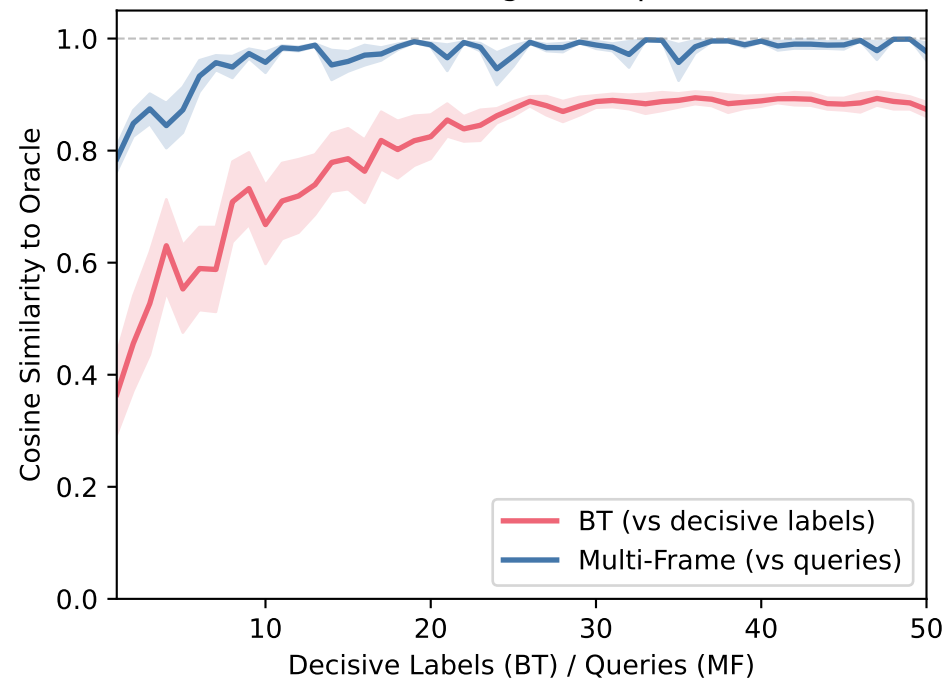
Protocol 2: Fixed Budget Comparison (K=50)
