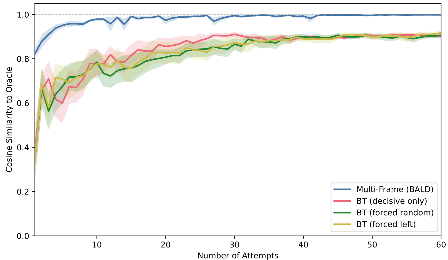
Protocol 3: BT Forced-Choice Variants ( \tau=\tau'=0.25 , 15 trials)
