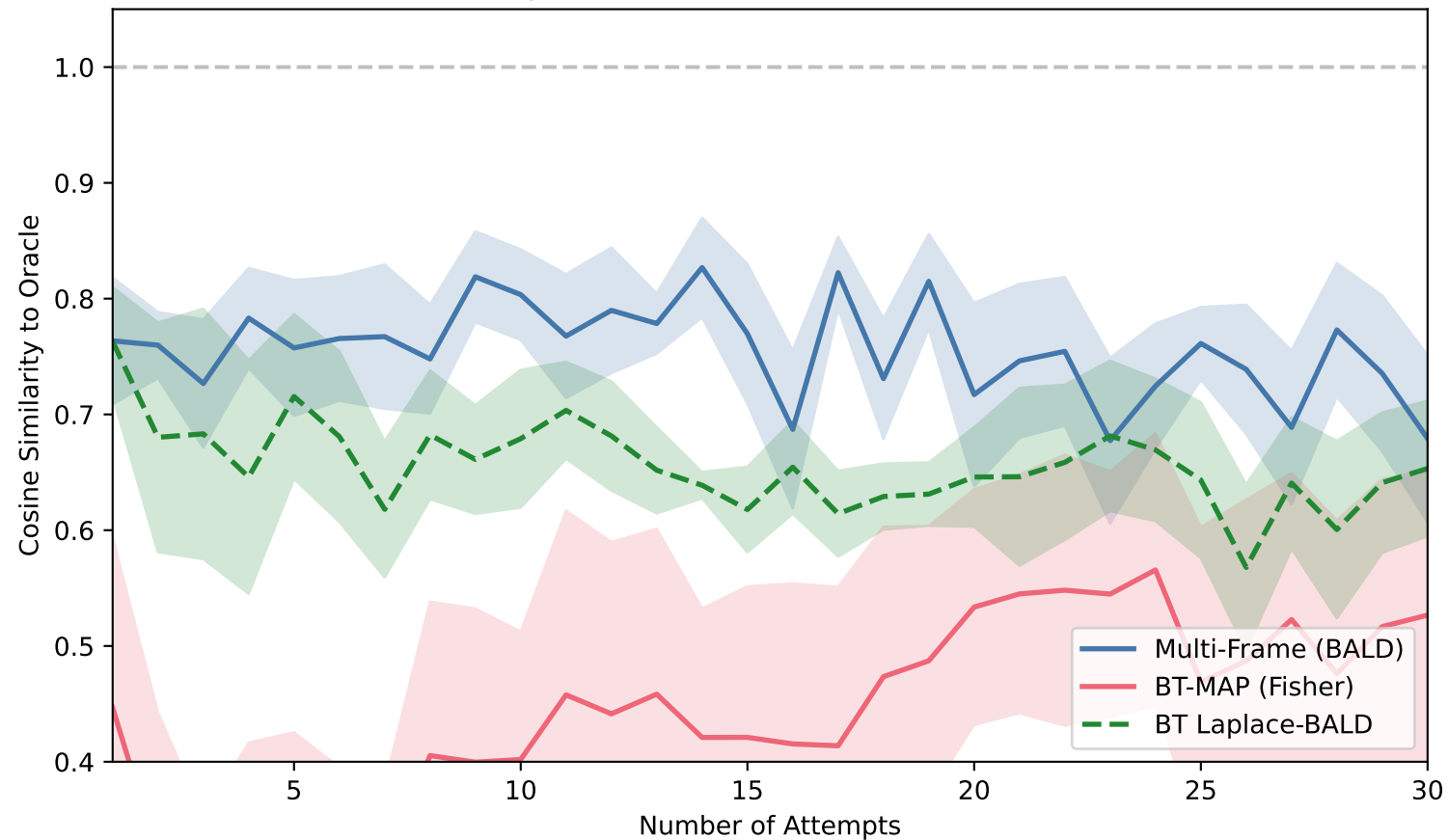
Sanity Test: \tau=\tau'=0 (All Decisive, 5 trials)
