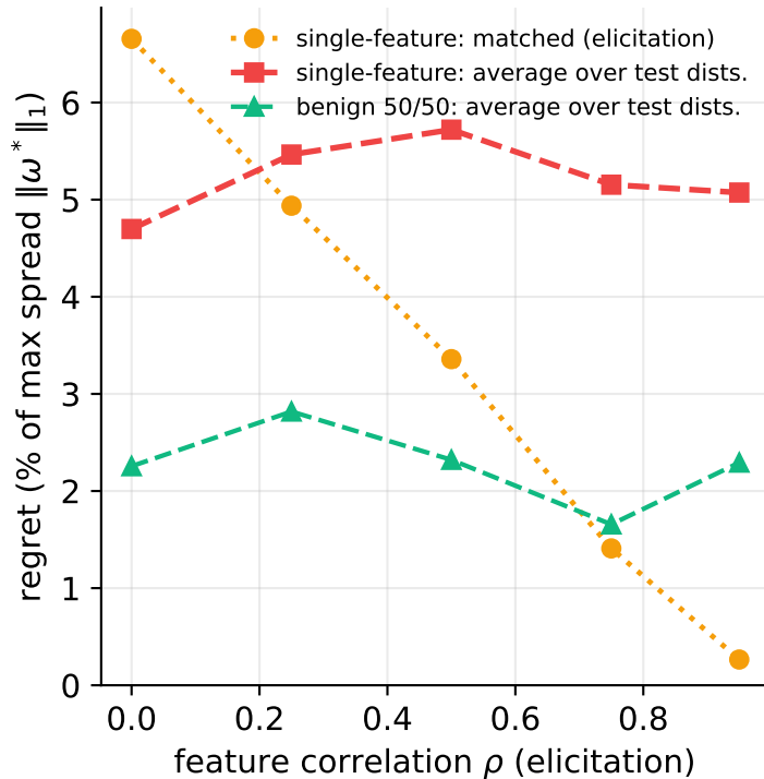
Matched regret is masked ( \rightarrow 0 ); average over test dists. persists ( \sim 2\times benign)
