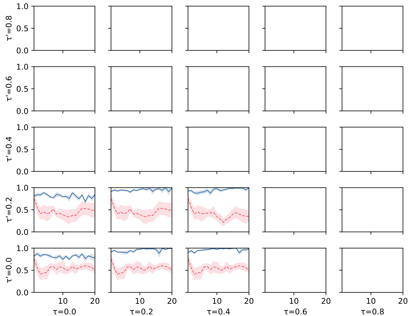
MF-MAP vs BT-MAP (Skips)
