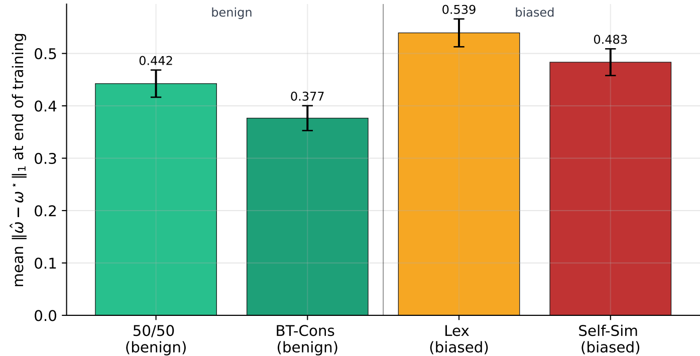
Block 1b: weight-error \ell_1 per forcing rule (mean \pm SE across oracles)
