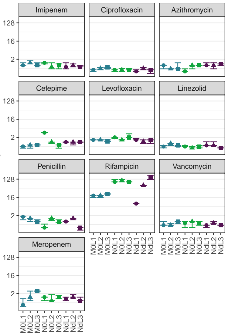
Fold Change MIC
