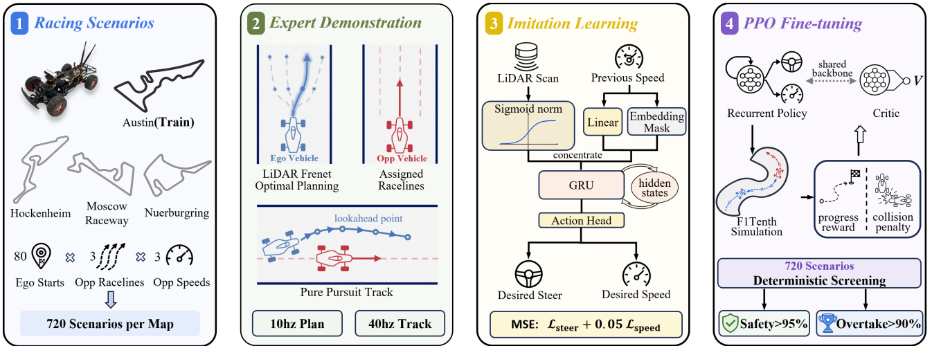
Fig. 2. System overview. The F1TENTH vehicle photograph in panel 1 is adapted from the official F1TENTH documentation under CC BY-NC-SA 4.0.
