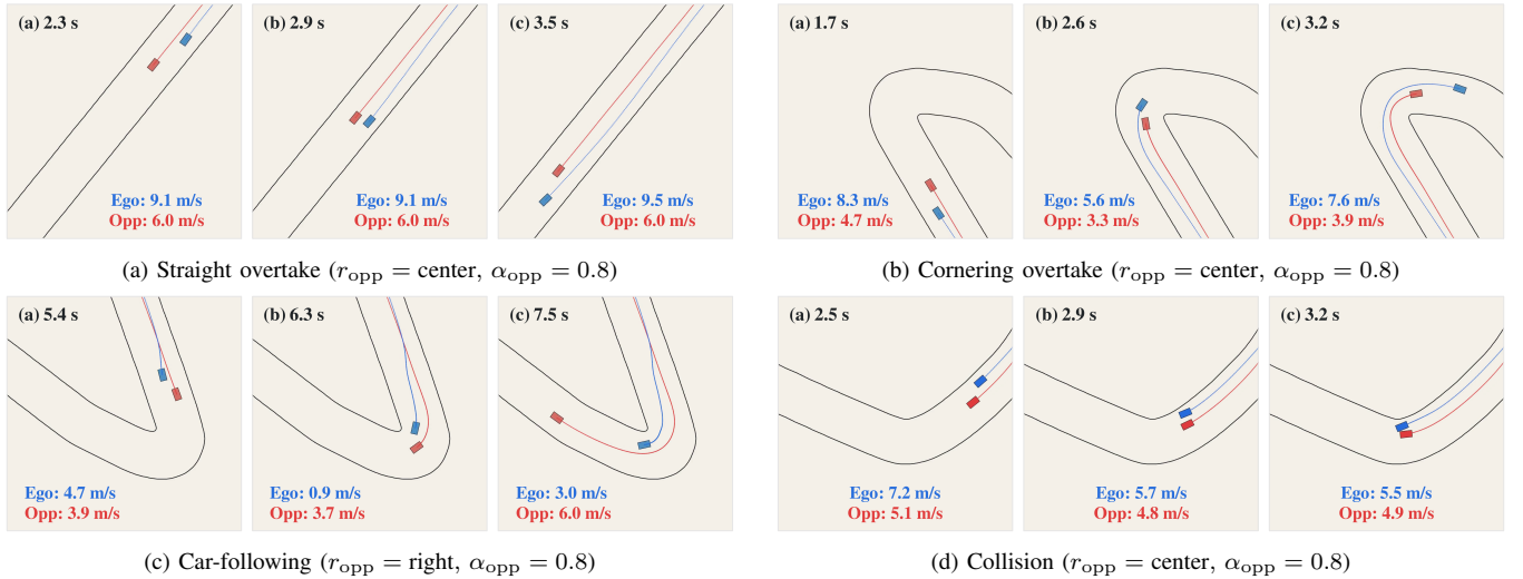
Fig. 5. Head-to-head scenarios on the Austin circuit. Blue and red denote the ego vehicle and opponent, respectively, with their trajectories rendered in matching colors.
