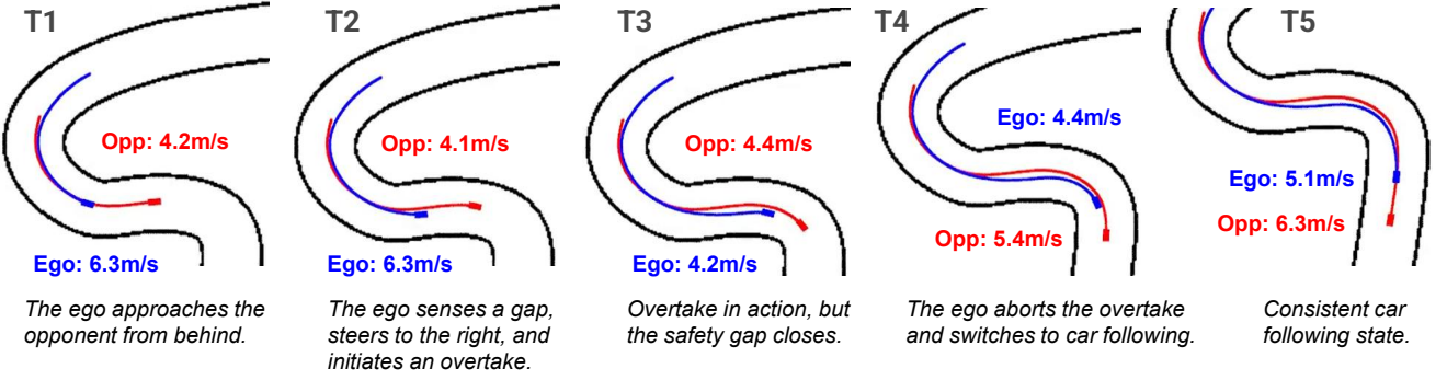
Fig. 5. Car-following example.
