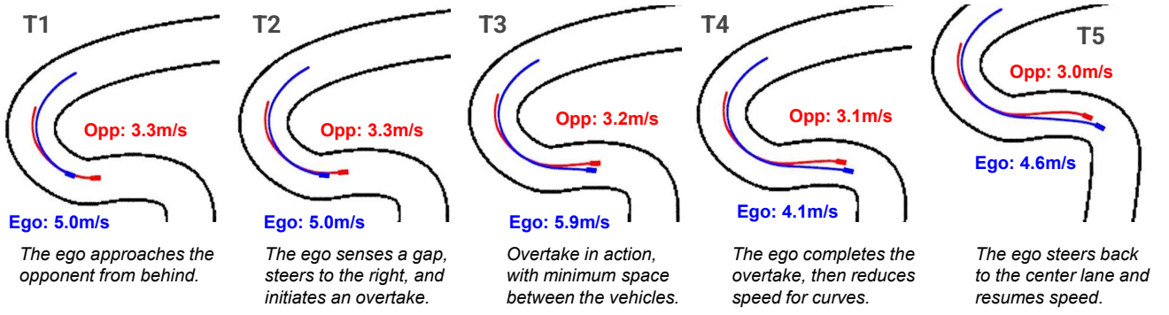
Fig. 4. Overtaking example.
