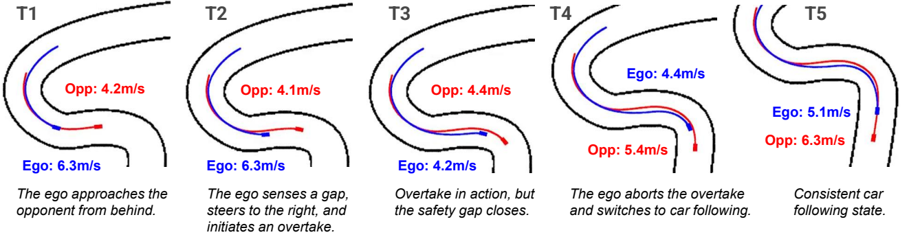
Fig. 5. Car-following example.
