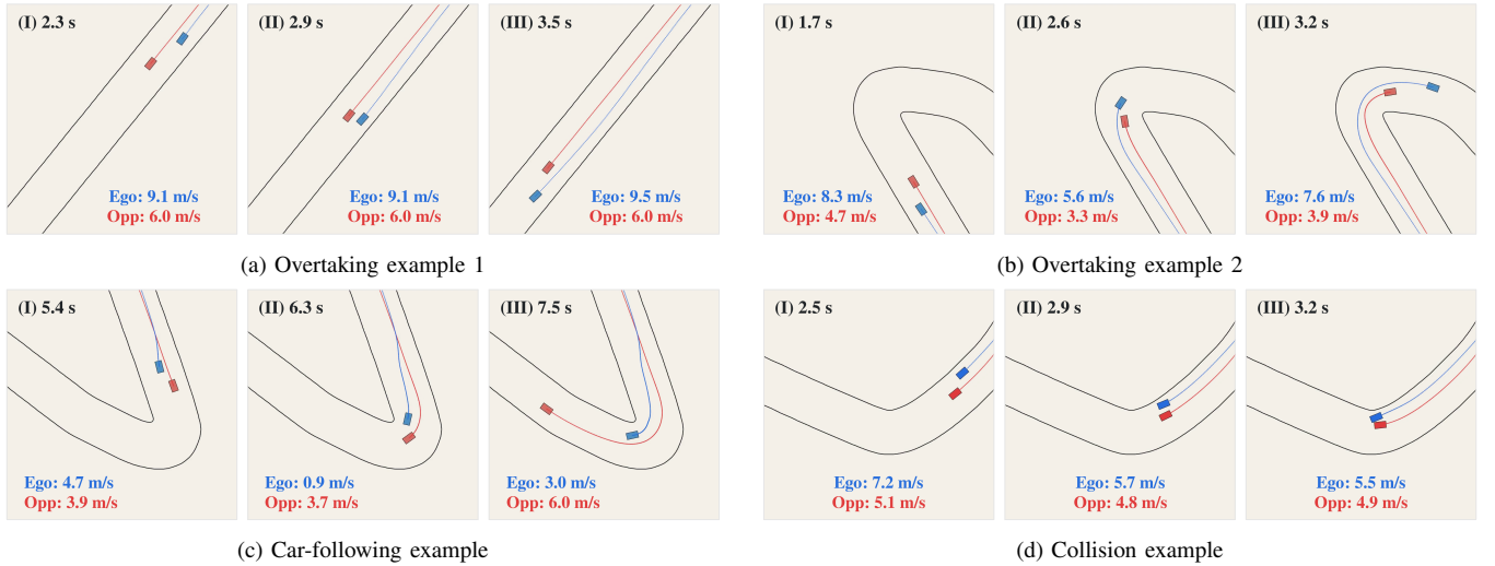
Fig. 5. Representative head-to-head racing outcomes. Each three-frame sequence is shown in temporal order from left to right. Blue denotes the ego vehicle and red denotes the opponent.
