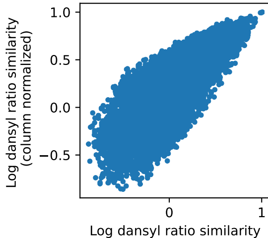
Spearman Correlation: X2n vs X2
