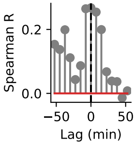
Adenine
