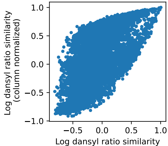
Spearman Correlation: X1n vs X1
