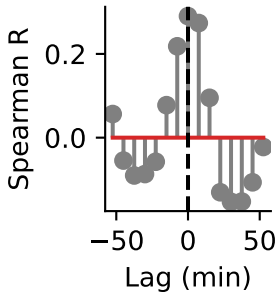
Taurine
