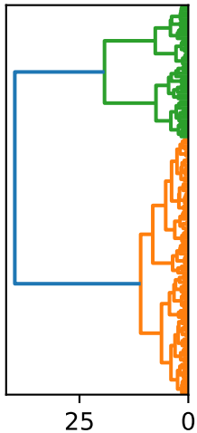
Dendrogram
