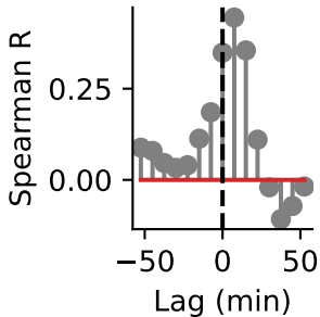
Creatine
