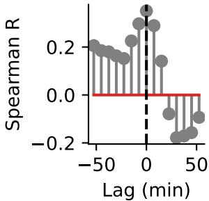
Thymine
