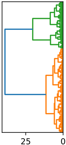
Dendrogram
