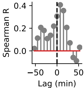
Valine
