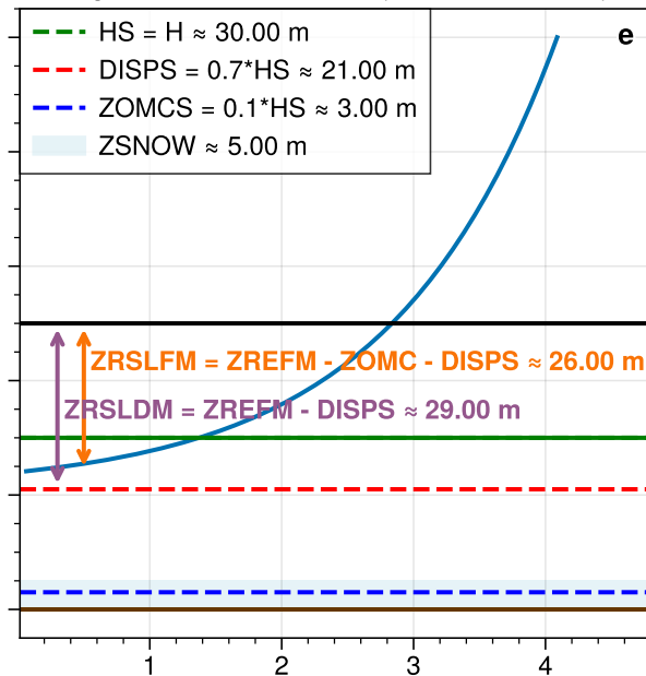
Logarithmic Wind Profile (Trees over snow)
