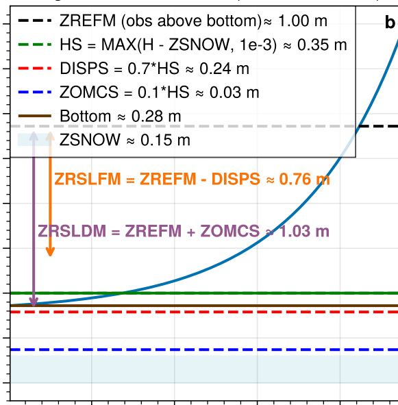
Logarithmic Wind Profile (Trees over snow)
