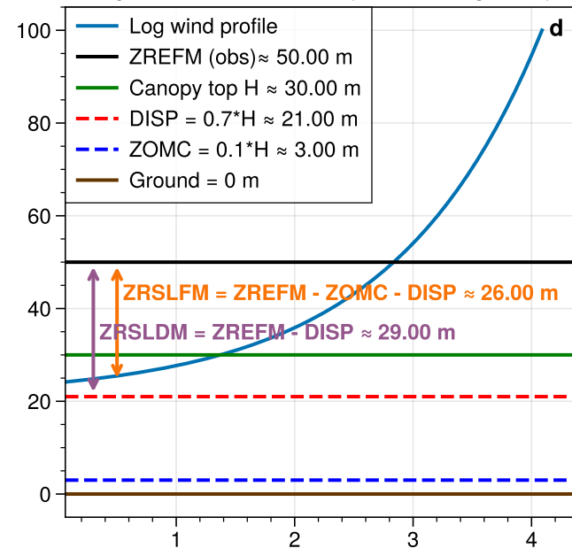
Logarithmic Wind Profile (Trees over ground)
