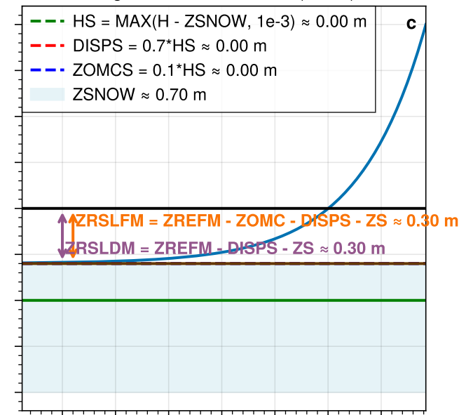
Logarithmic Wind Profile (Snow)
