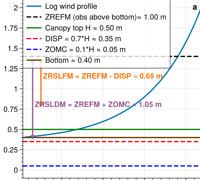
Logarithmic Wind Profile (Trees over ground)
