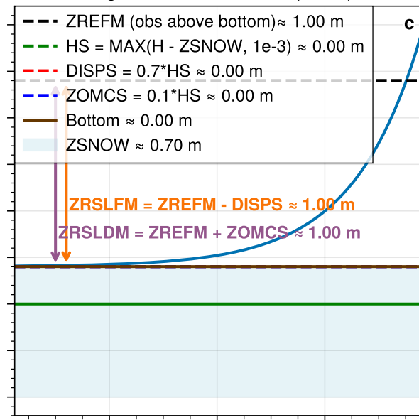
Logarithmic Wind Profile (Snow)
