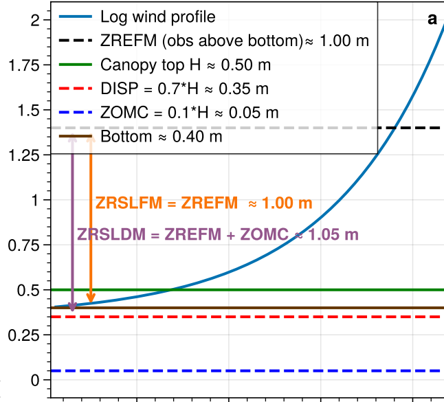
Logarithmic Wind Profile (Trees over ground)
