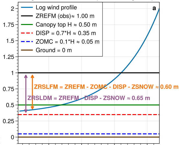
Logarithmic Wind Profile (Trees over ground)
