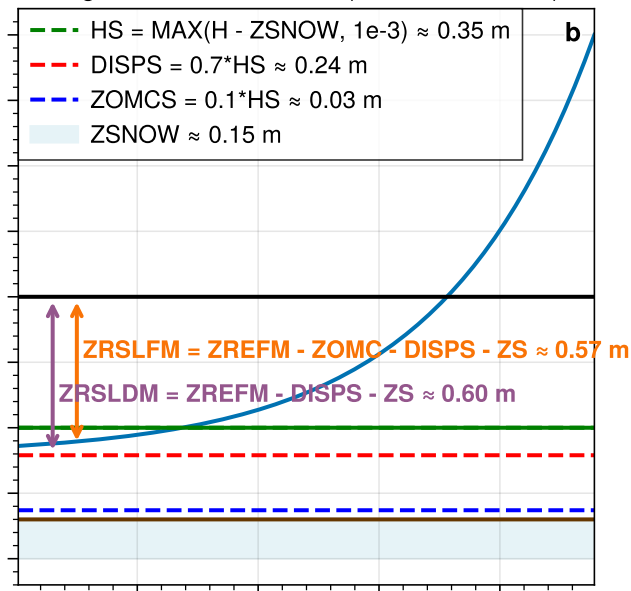
Logarithmic Wind Profile (Trees over snow)
