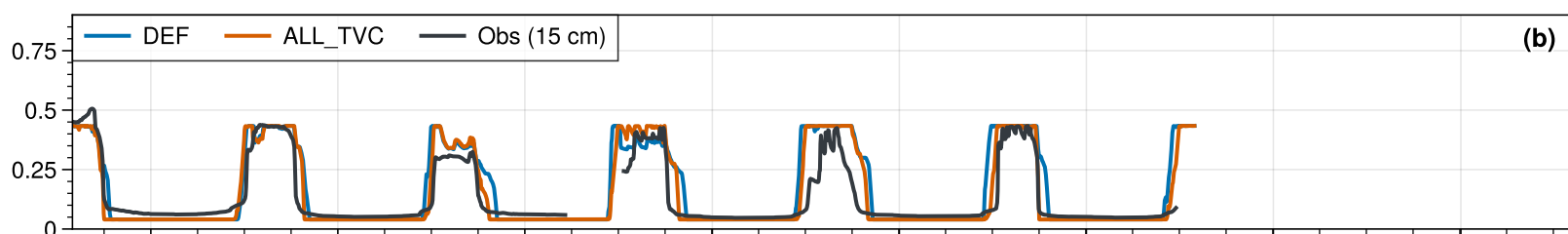
Umiujaq TUNDRA, northeastern Canada (2015-08 - 2021-07)
