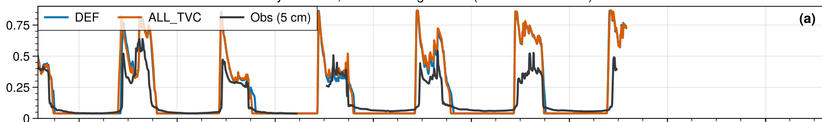
Bylot Island, Canadian high Arctic (2013-08 - 2019-07)
