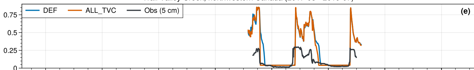
Trail Valley Creek, northwestern Canada (2017-08 - 2019-07)
