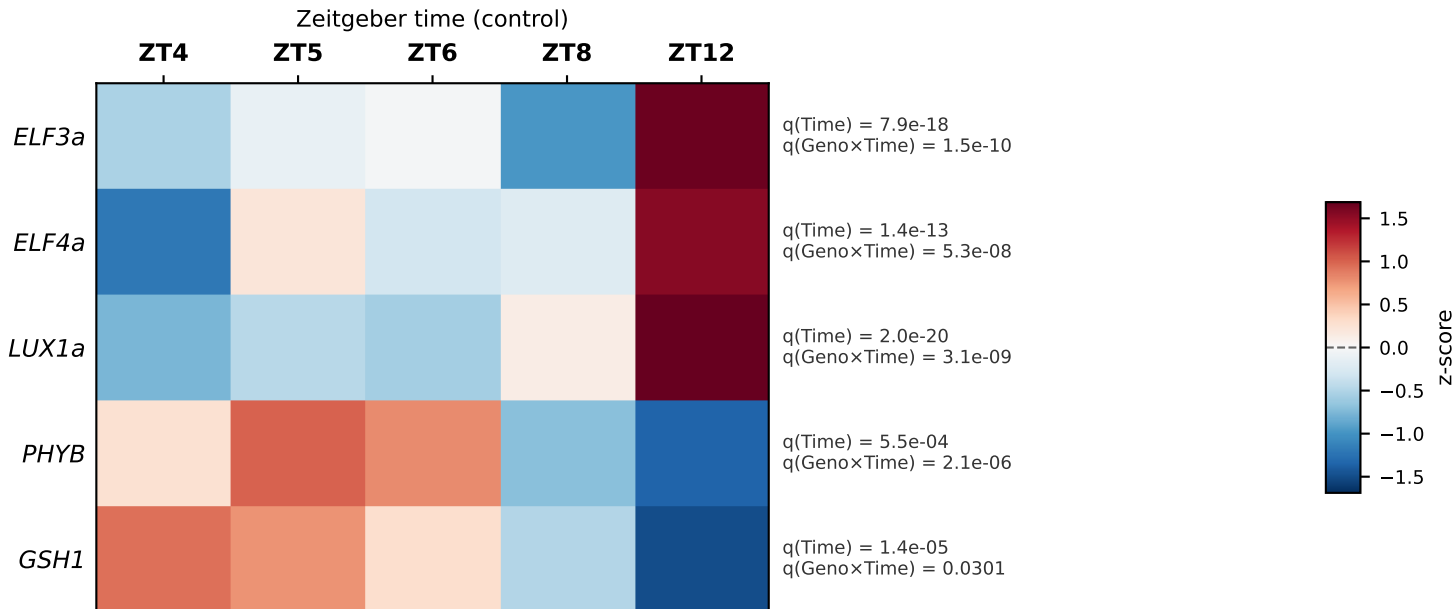
Circadian candidate genes — V.vi control conditions Vitis vinifera cv. Cabernet Sauvignon (Hopper et al. 2016, BMC Plant Biol) Colour: z-score per gene across time-point means | q-values: BH-FDR 3-way ANOVA (full dataset)
