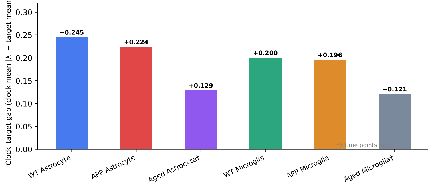
Figure S2. Clock-target gap across all six conditions Positive = clock above target (hierarchy maintained); gap narrows with age/disease
