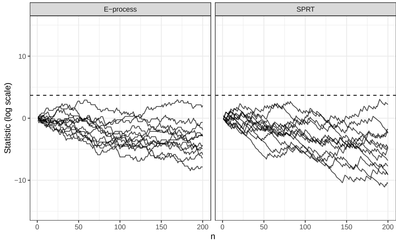
E-process and SPRT trajectories under H_0
