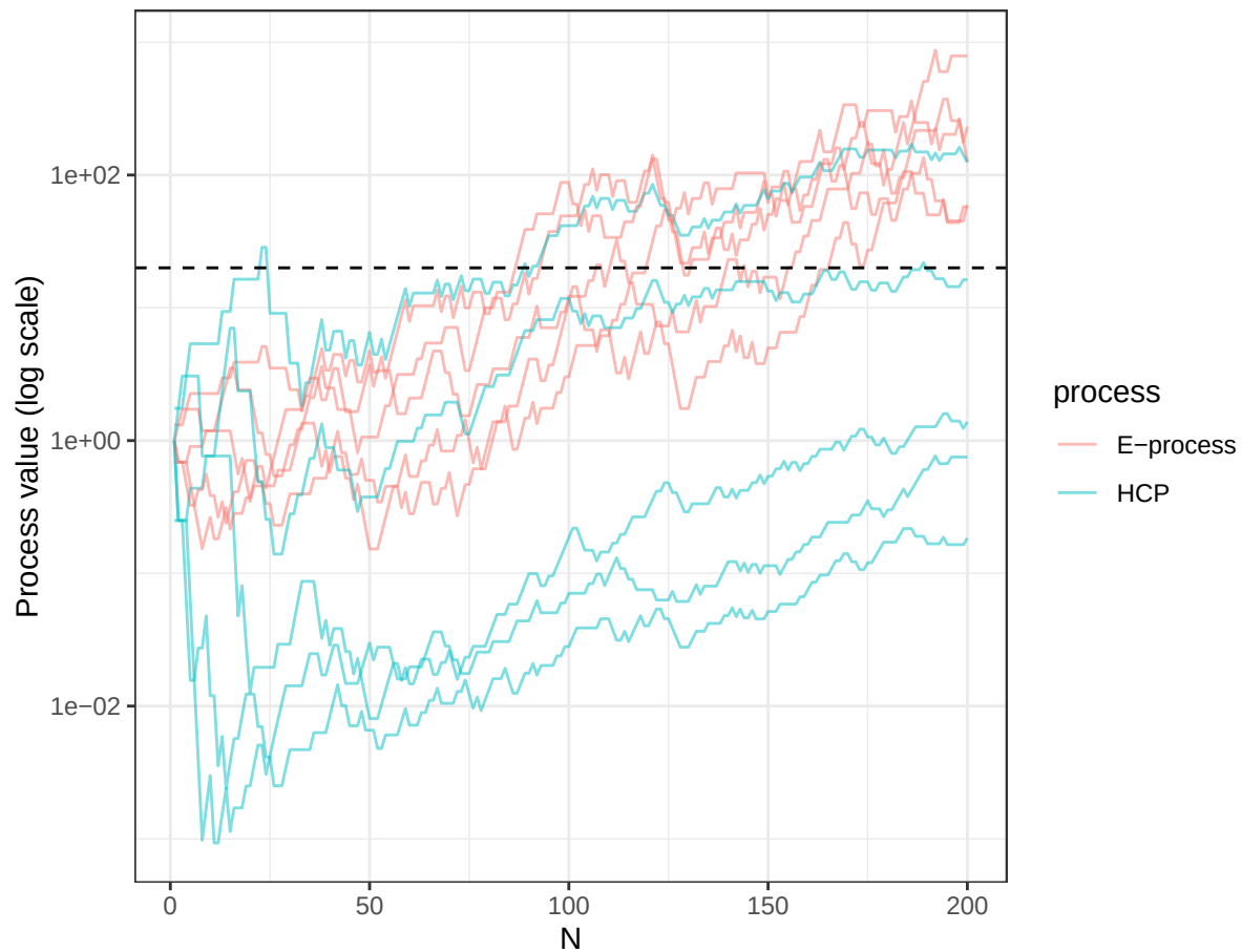
5 simulated paths (overlay)
