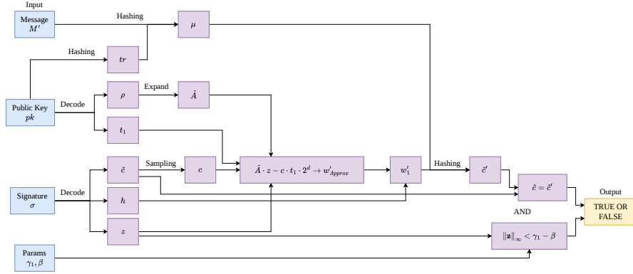
Fig. 8: ML-DSA Internal Verification Algorithm ML-DSA.Verify_internal
