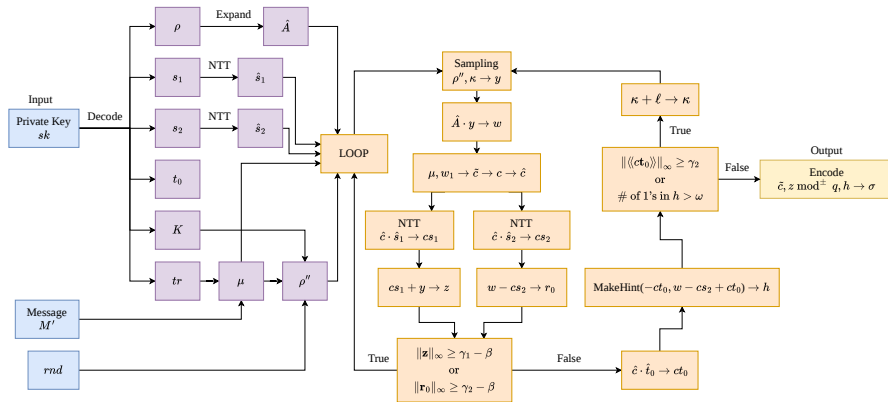
Fig. 7: ML-DSA Internal Signing Algorithm ML-DSA.Sign_internal
