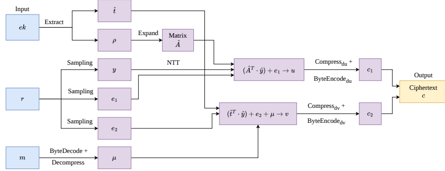
Fig. 3: Kyber Encryption Algorithm K-PKE.Encrypt
