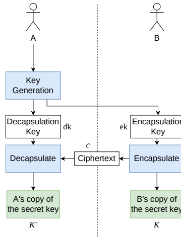
Fig. 1: Simplified key establishment process using KEM
