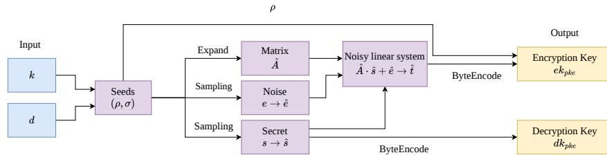
Fig. 2: Kyber Key Generation Algorithm K-PKE.KeyGen
