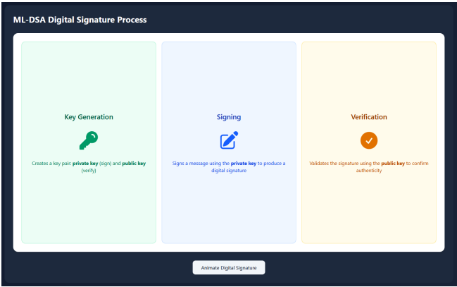
Fig. 11: ML-DSA Process
