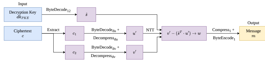
Fig. 4: Kyber Decryption Algorithm K-PKE.Decrypt
