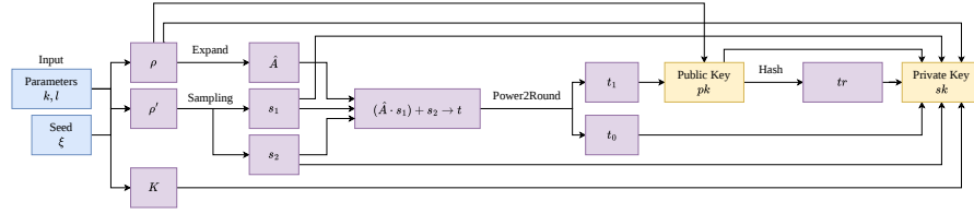
Fig. 6: ML-DSA Internal Keygen Algorithm ML-DSA.KeyGen_internal
