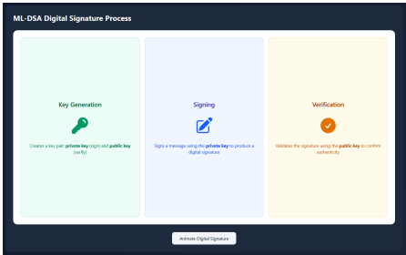
Fig. 11: ML-DSA Process
