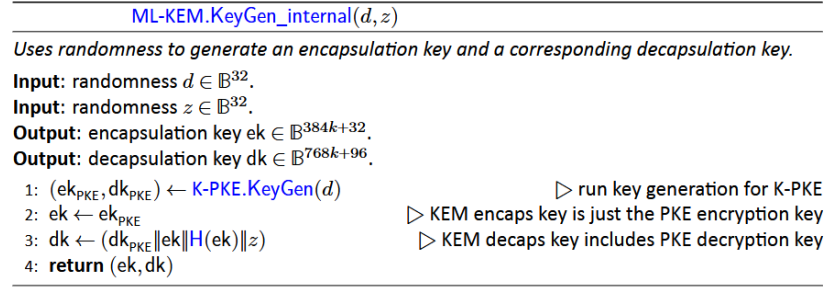
Fig. 3: ML-KEM.KeyGen\_internal() algorithm. Sourced from [16].
