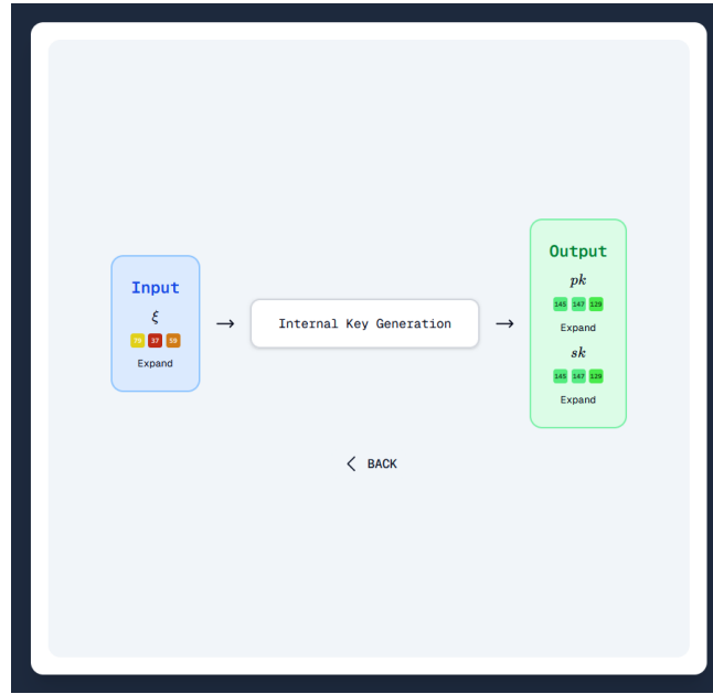
Fig. 24: ML-DSA Full Animation Section
