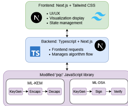
Fig. 18: Latviz fullstack architecture
