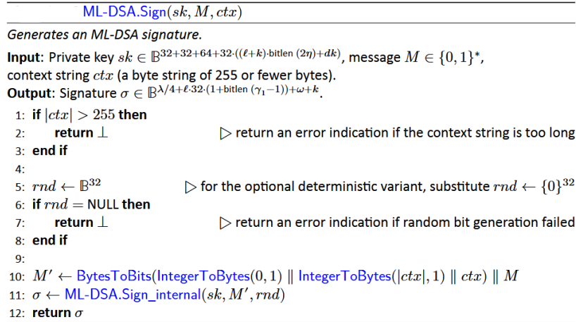
Fig. 14: ML-DSA.Sign() algorithm. Sourced from [15].
