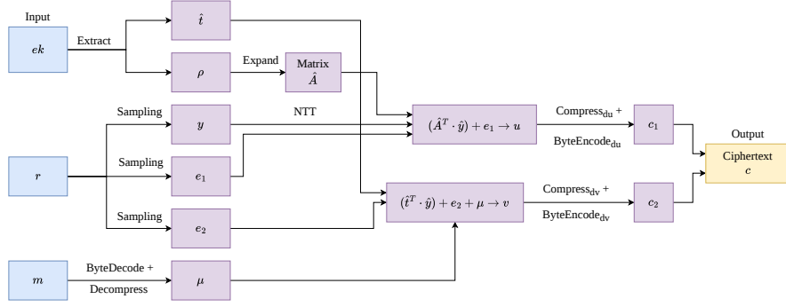
Fig. 7: Kyber Encryption Algorithm K-PKE.Encrypt
