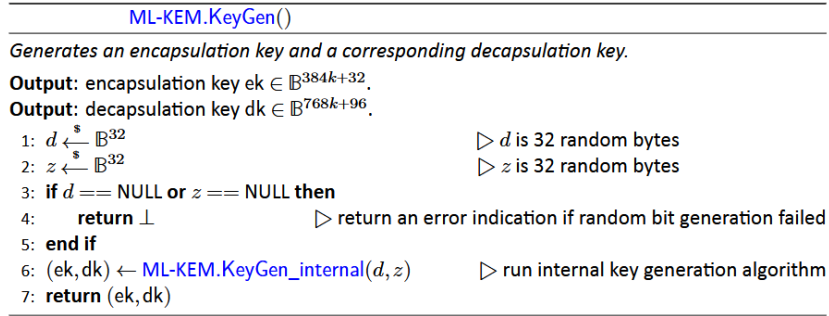
Fig. 2: ML-KEM.KeyGen() algorithm. Sourced from [16].
