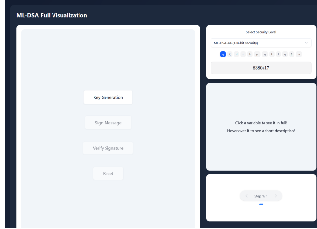
Fig. 22: ML-DSA Full Animation Section
