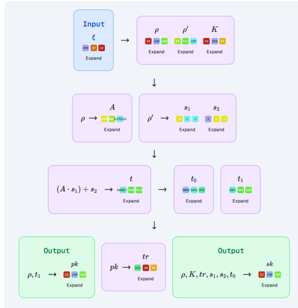
Fig. 31: ML-DSA Full Animation Section (Step 9)
