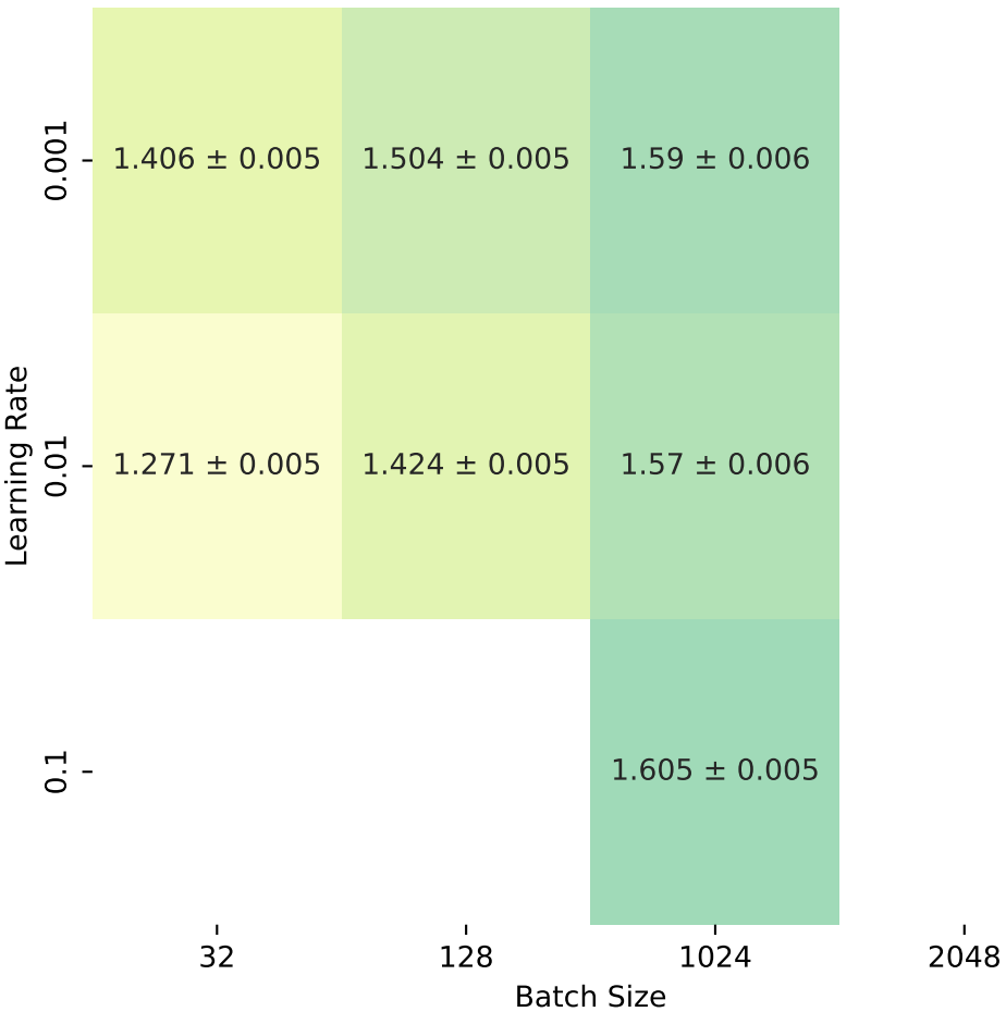
Tagging Power Before Calibration (simple)
