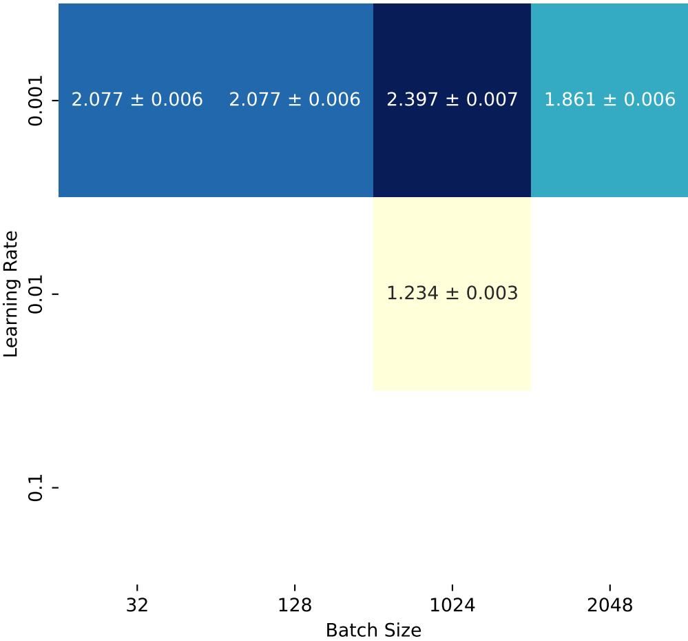
Tagging Power Before Calibration (complex)
