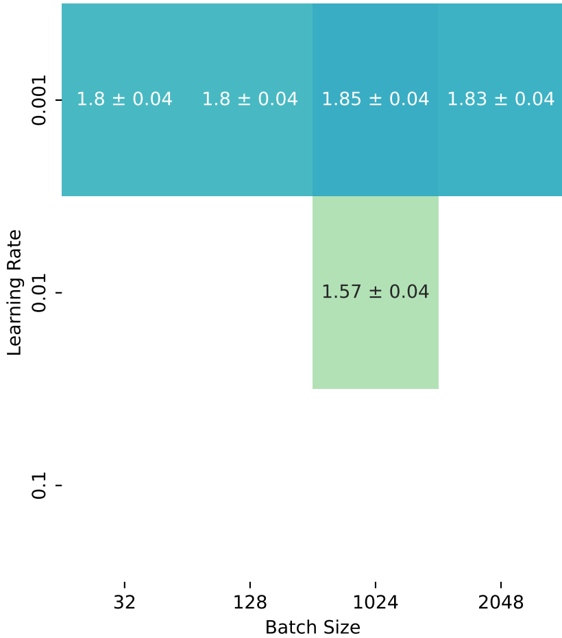
Calibrated Tagging Power with Logit(complex)
