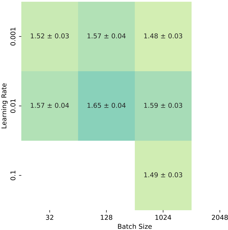
Calibrated Tagging Power with mistag (simple)
