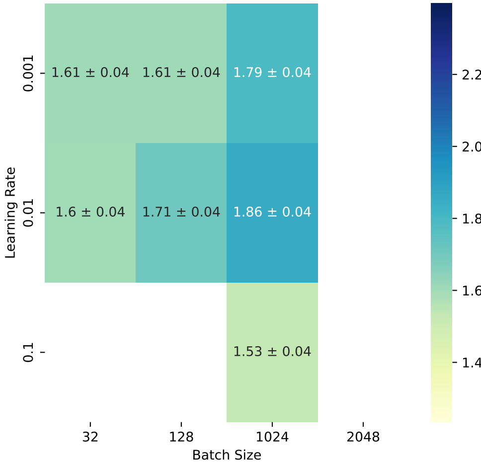
Calibrated Tagging Power with Logit(simple)
