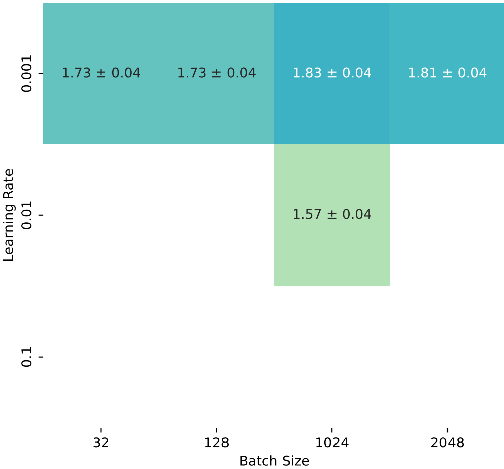
Calibrated Tagging Power with mistag (complex)
