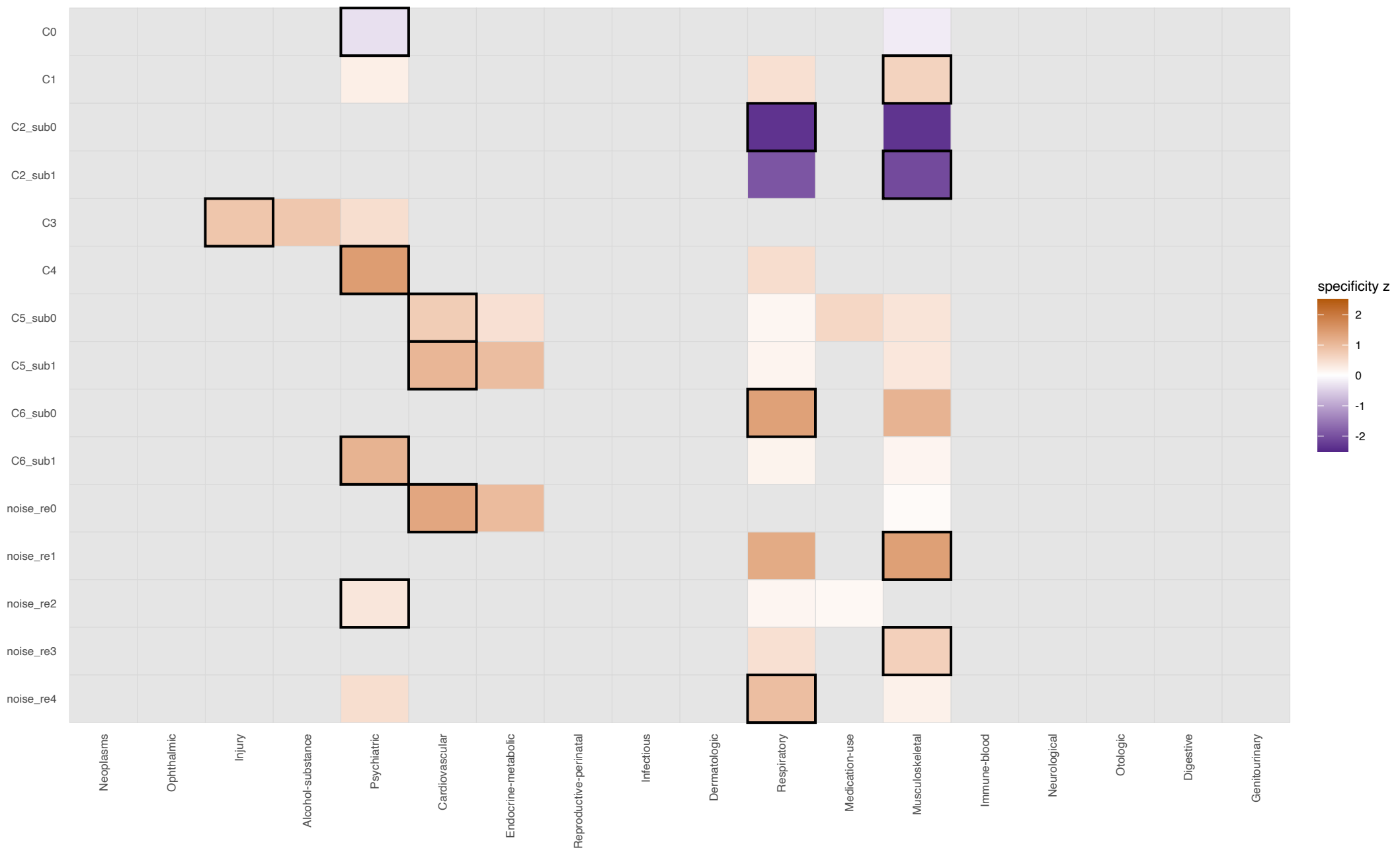
Cluster specificity — disease track z of pooled rg within each category across clusters (grey = not significant; box = most distinctive)
