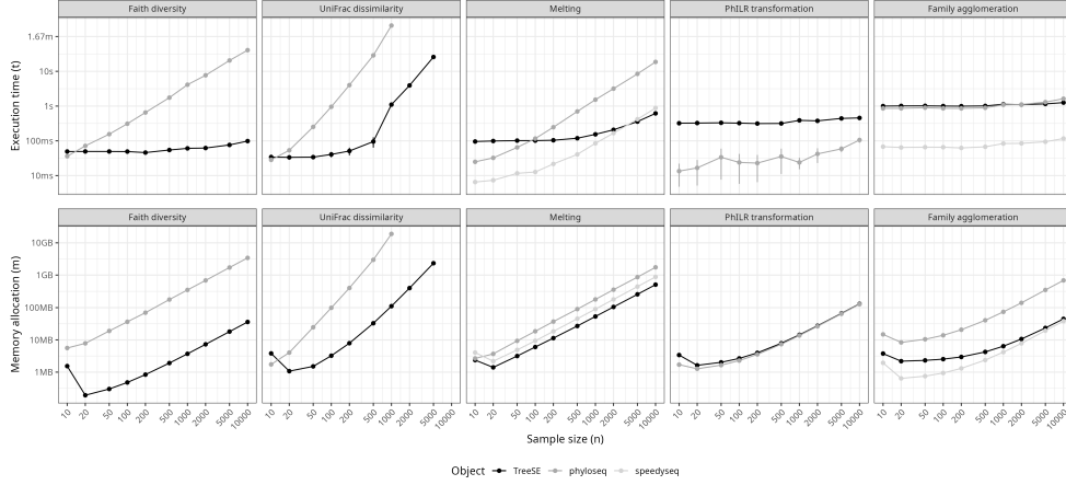
Figure 3: Benchmarking mia/TreeSE against phyloseq and speedyseq. The TreeSE ecosystem outperforms phyloseq overall. While speedyseq is faster in certain operations, TreeSE scales more efficiently in both memory usage and computation time.
