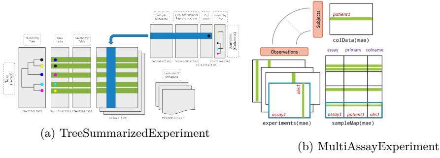
Figure 2: Bioconductor data containers for microbiome data. (a) TreeSummarizedExperiment (TreeSE) . TreeSE supports hierarchical and multi-table analysis in microbiome data science 23 . It links the numeric abundance matrix and potential alternative versions (statistical transformations, different taxonomic levels, dimensionality reduction) with tabular and hierarchical side information on the features (rows) and samples (columns). Additional slots for reference sequences and experiment metadata are available. (b) MultiAssayExperiment (MAE) . MAE facilitates integration of data from multiple experiments 24 .
