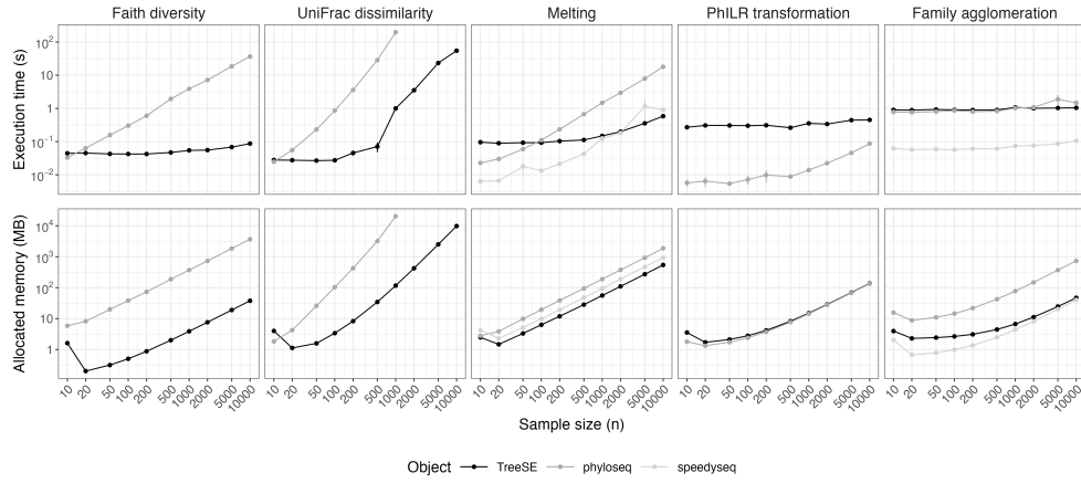
Figure 3: Benchmarking mia/TreeSE against phyloseq and speedyseq. TreeSE, phyloseq and speedyseq were benchmarked for five common analytical operations applied to random subsets of samples from the GrieneisenTSDData experiment 25 . Overall, the TreeSE methods outperformed phyloseq. While speedyseq was faster in certain operations, TreeSE scaled more efficiently in both execution time (s) and allocated memory (MB) with increasing sample size (n).
