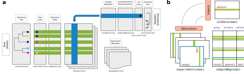
Figure 2: Bioconductor data containers for microbiome data. (a) TreeSummarizedExperiment (TreeSE) . TreeSE supports hierarchical and multi-table analysis in microbiome data science 23 . It links the numeric abundance matrix and potential alternative versions (statistical transformations, different taxonomic levels, dimensionality reduction) with tabular and hierarchical side information on the features (rows) and samples (columns). Additional slots for reference sequences and experiment metadata are available. (Figure modified from 23 ) (b) MultiAssayExperiment (MAE) . MAE facilitates integration of data from multiple experiments 24 . (Figure from 24 )
